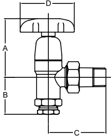
15mm & 1/2" Angle
