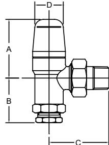
15mm & 1/2" Angle
