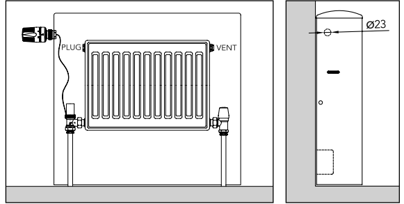
Close Coupled Kit
